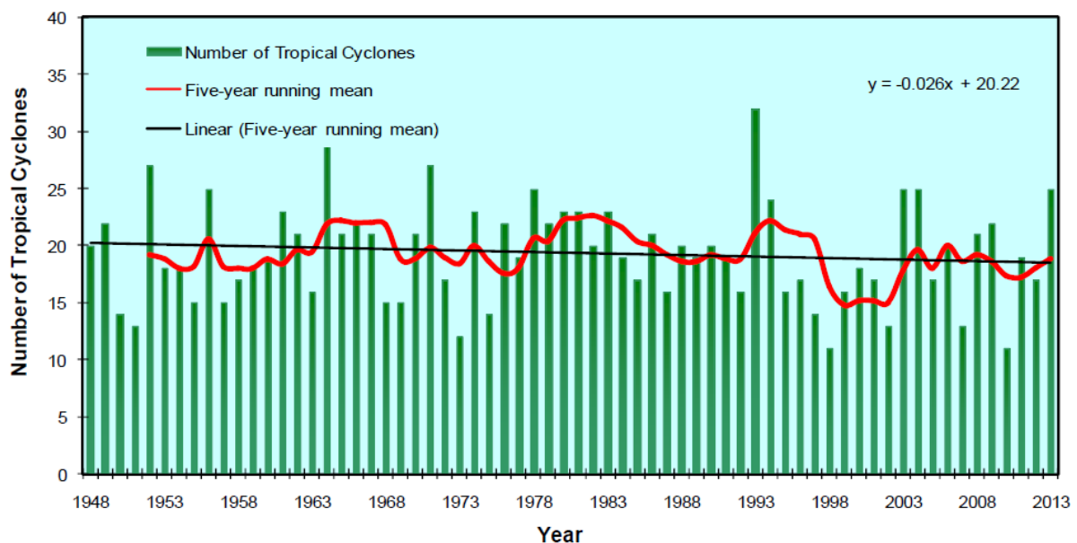
Annual Number of Tropical Cyclones in the PAR Period: 1948-2013
